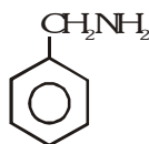
Phenyl methanamine (Benzylamine)
