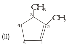
2,3-Dimethyl cyclopent-1-ene
