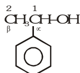
1-phenyl ethanol ( \alpha -phenyl ethyl alcohol)
