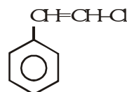
1-chloro-2-phenyl ethene
